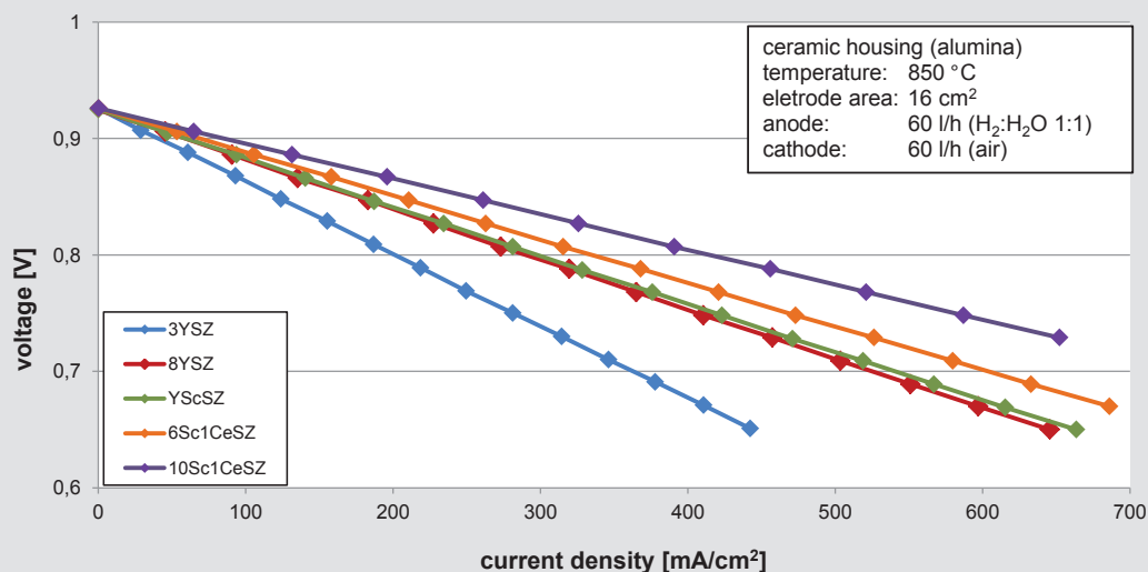
KeraCell II - typical electrode performance
