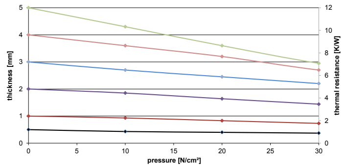
Compression 86/200
